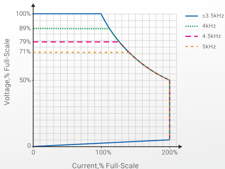
High frequency derating curve
